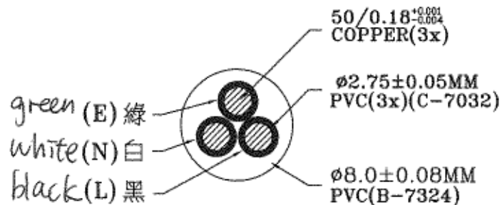
X-X CROSS-SECTION
